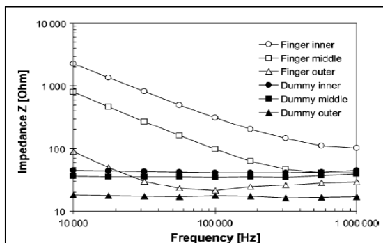
Fig 7: Measured Impedance Modulus Response for one Live Finger and Fake Finger
