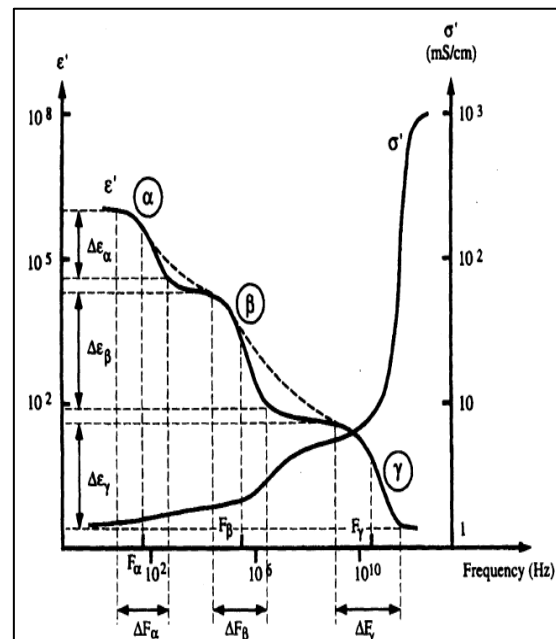
Fig 2: Dispersion of Conductivity and Permittivity
