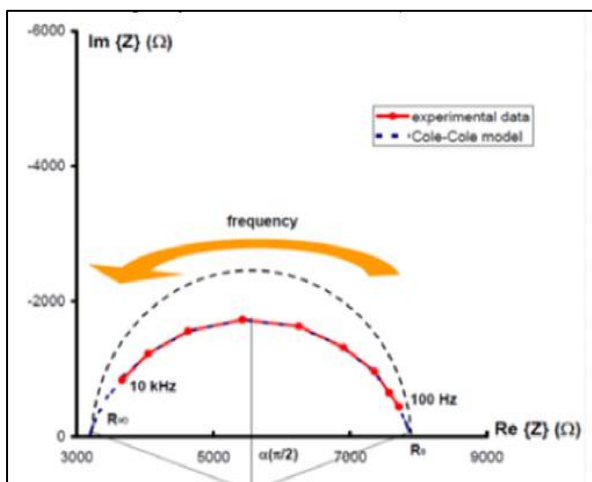
Fig 3: Wessel Diagram of an Actual Bioimpedance Measurement and the Superimposed Cole Model Results.
